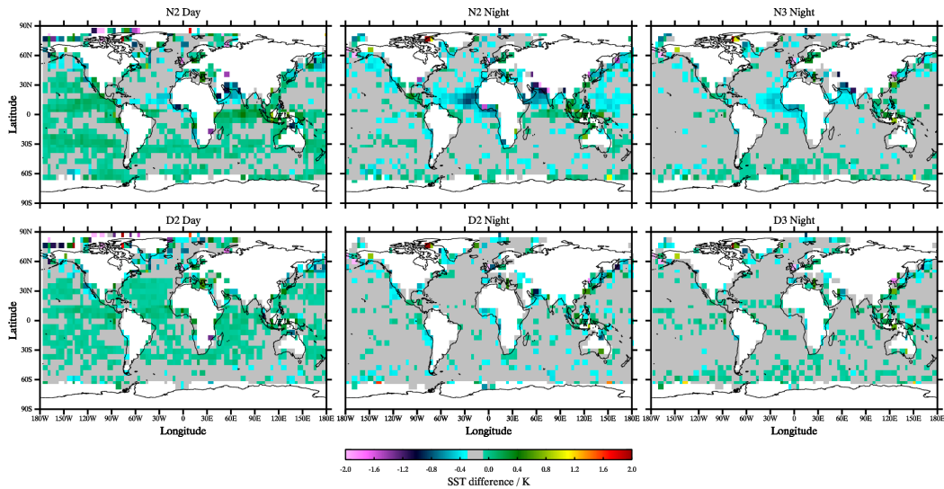
Figure 7-2: Spatial distribution of the median discrepancy between AATSR NR SST skin and drifter SST depth . The greyed region indicates a band of +/- 0.1 K around the expected mean skin offset of -0.17 K.
