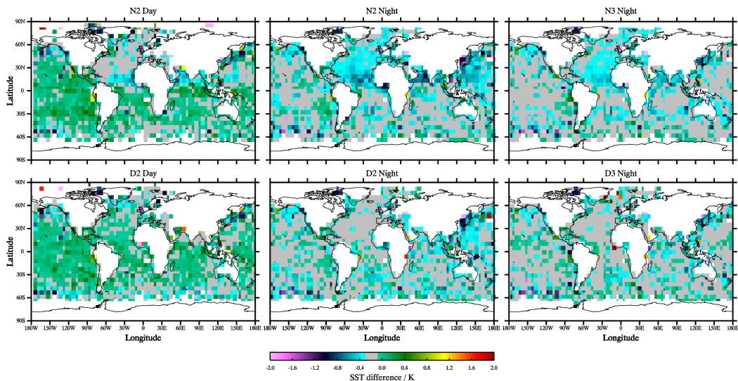
Figure 8-2: Spatial distribution of the median discrepancy between ATSR-2 NR SST skin and drifter SST depth . The greyed region indicates a band of +/- 0.1 K around the expected mean skin offset of -0.17 K.
